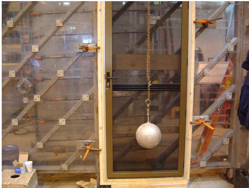
Photo No. 1 Test Setup of Impact Test
